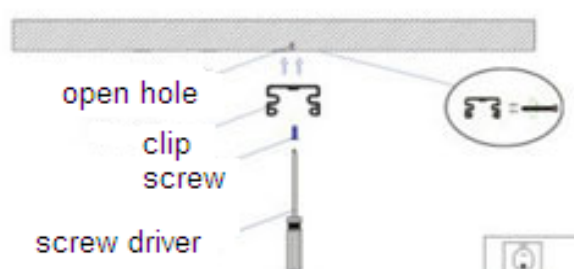
B. Screw the clip on the ceiling tightly
